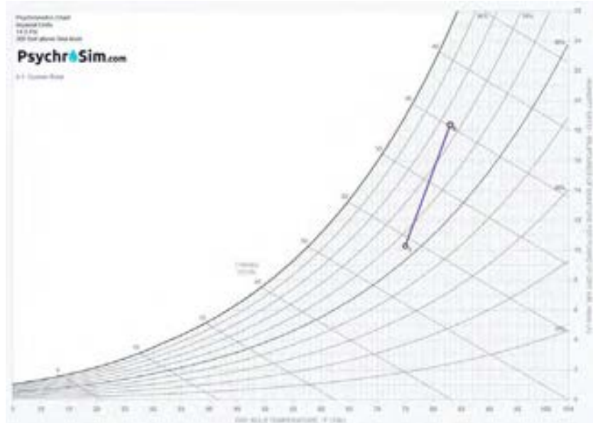
Figure 7: Cooling Process
