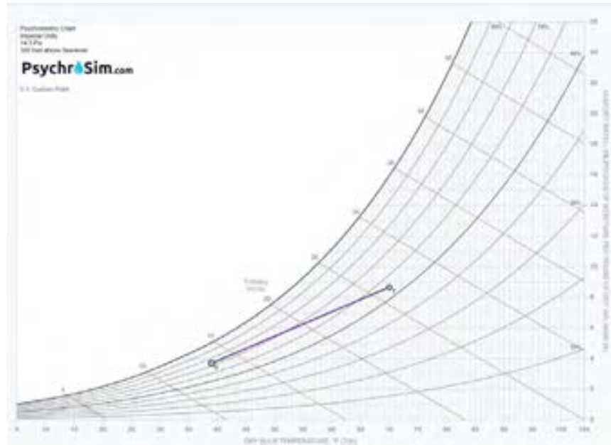
Figure 8: Heating Process
