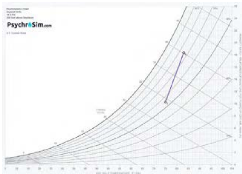
Figure 7: Cooling Process
